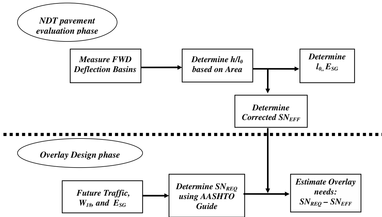
FIGURE 6 Flowchart of the YONAPAVE Method
