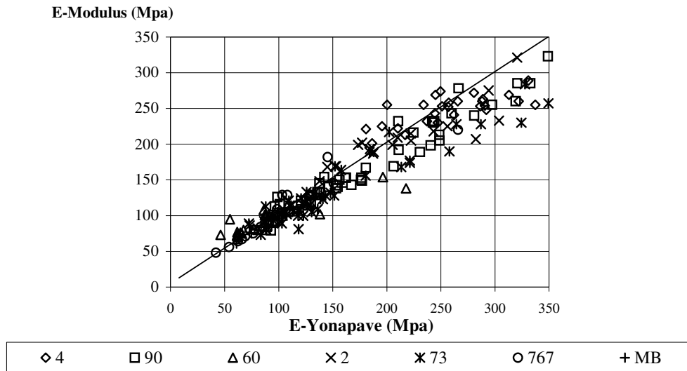
FIGURE 4 E_{SG} MODULUS vs. E_{SG} YONAPAVE
